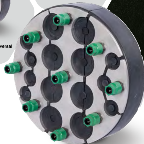
KRASO® Sealing Insert Universal Multiple - split - 200 Design 2
